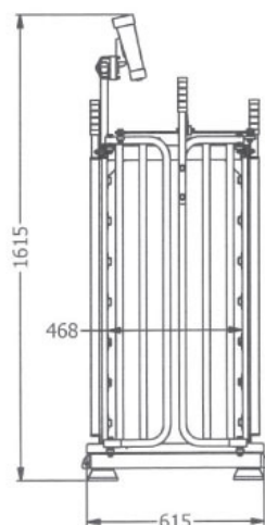
C11350 3 Way Calf Weigh Crate
